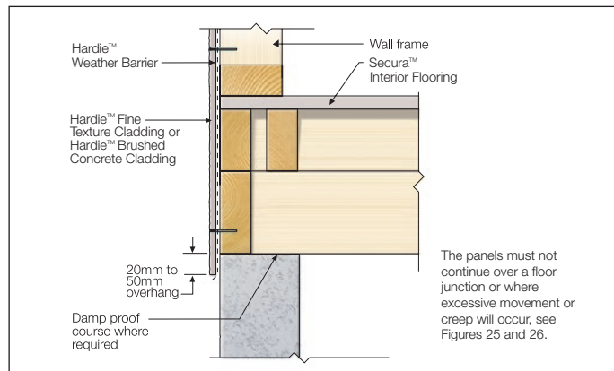
FIGURE 5 LOWER FLOOR JUNCTION
